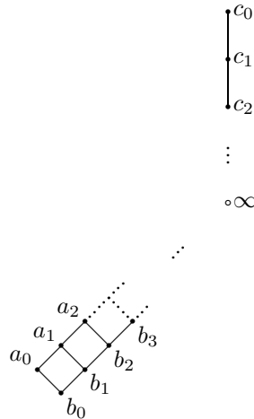
FIGURE 3. The lattice \overline{F} .
