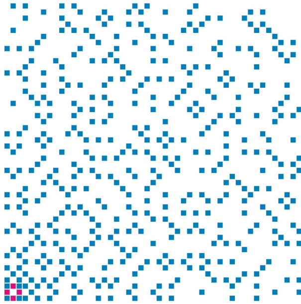
Primes Units Q(V-3) class 1 chi o+o
