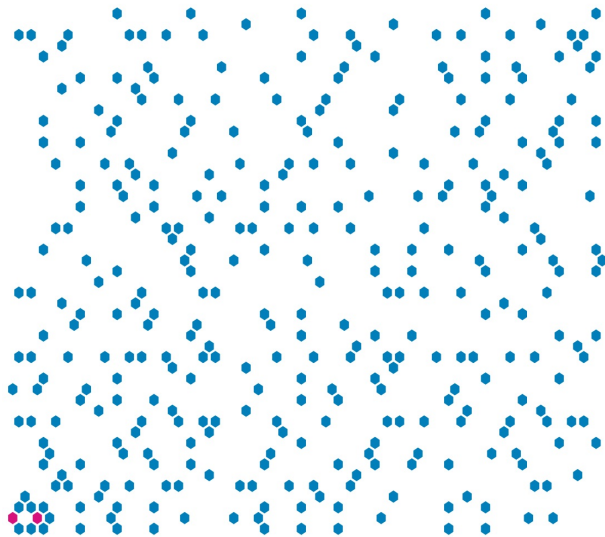
Primes Units Q(V-11) class 1 chi o+----++-o
