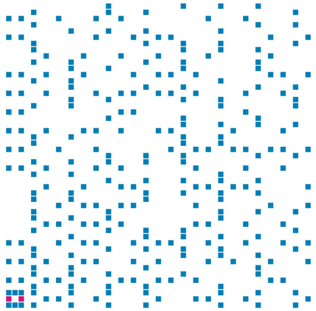
Primes Units Q(V-7) class 1 chi o+----o
