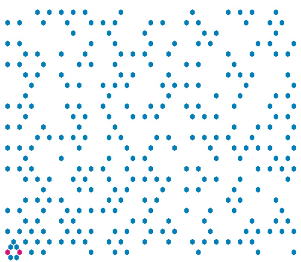
Primes Units Q(V-7) class 1 chi o+----o
