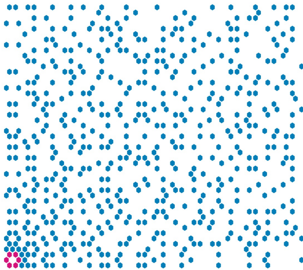
Primes Units Q(V-3) class 1 chi o+o
