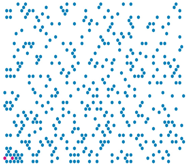
Primes Units Q(V-19) class 1 chi o+----++-o
