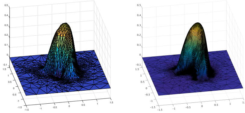
FIGURE 2. Approximations u_{\tau_{i,K}}^{\lambda_{\sigma_i}^{(K-1)}} for i = 3 (left) and i = 6 (right) produced with K = 6 , \zeta = \sqrt{2} , \theta = 0.1 .
