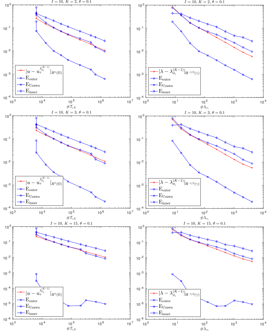
FIGURE 5. Errors |u - u_{\tau_i, K}^{\lambda_i^{(K-1)}}|_{H^1(\Omega)} (left) and \|\lambda - \lambda_{\sigma_i}^{(K-1)}\|_{H^{-1/2}(\gamma)} (right), and estimators for \zeta = \sqrt{2} , \theta = 0.1 , and K = 2 (top), K = 3 (middle) and K = 15 (bottom).
