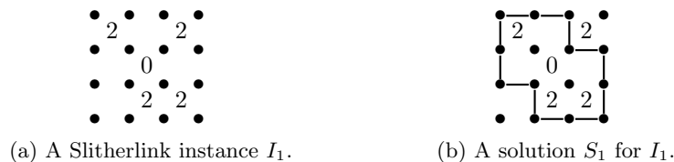
Figure 1: An example of a Slitherlink instance and a solution.
