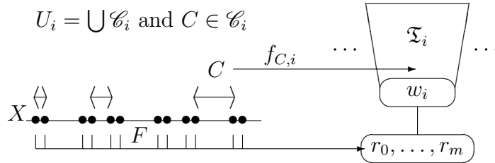
FIGURE 3. The mapping f : X \rightarrow \mathfrak{T} .
