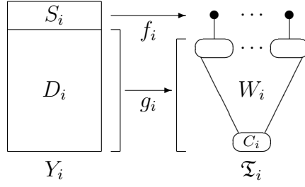
FIGURE 8. Extending g_i to f_i .
