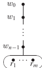
FIGURE 2. The \mathbf{S4}_{n+1} -frame \mathfrak{F}_m^n .
