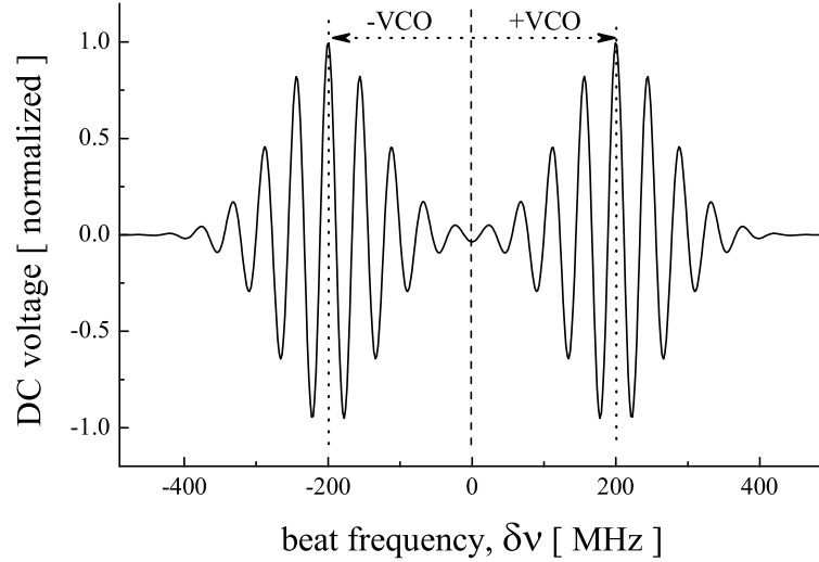
Figure 3.6: Qualitative representation of the locking signal for the phase contrast imaging laser. One of the two signals alone, centered around \delta\nu = 0\text{MHz} , would sketch the locking signal of the TIGER. A low-pass filter avoids overlap of the two signals. In reality the signal drops sharply to zero at zero beat frequency and at both centers of the shifted wrapping signals, as the mixer electronics do not transmit DC signals.
