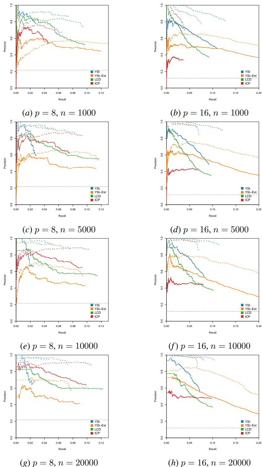
Figure 9: (Random Graphs, varied n ) PR curves for experiments with small ( p = 8 ) and large ( p = 16 ) random graphs for various sample sizes. Solid lines indicate performance using data under selection bias \mathcal{D}_S , while dashed lines show the performance for data where the selection mechanism is disabled \mathcal{D}_\emptyset .
