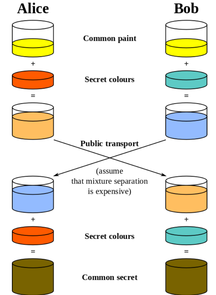
Diffie-Hellman Key Exchange Using Buckets of Paint Image credit: wikimedia.org .
