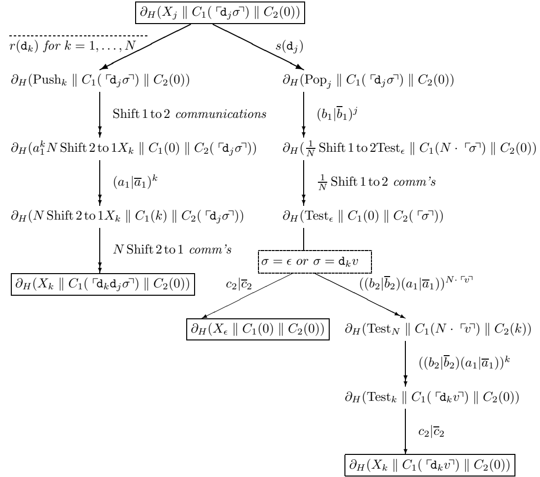
Figure 1: Calculations with \partial_H(X_j \parallel C_1(\lceil \mathbf{d}_j \sigma^\lceil) \parallel C_2(0)) .
