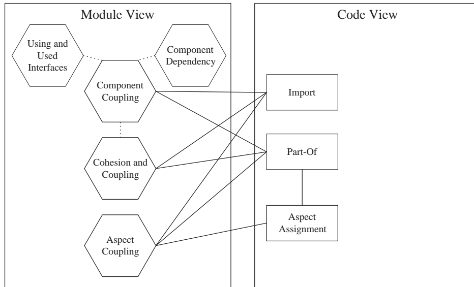
Figure 5.2: Overview of Redefined Architecture
