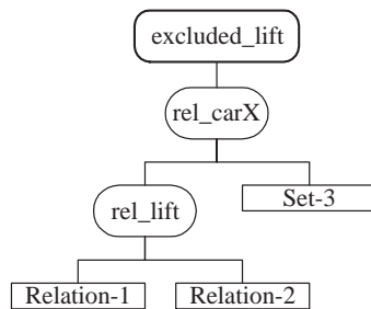
Figure B.1: High Level Operations
