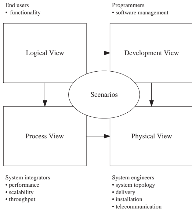
Figure 1.2: The 4+1 View Model
