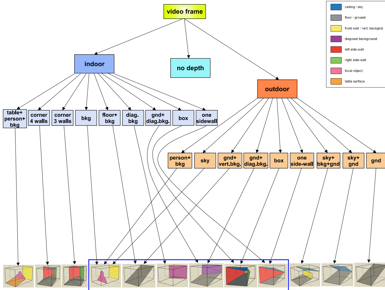
Figure 2. The original classification of TRECVID key-frames into stage types, inspired by Hoiem et al. [9] - the top-level categorization is into indoor and outdoor scenes, as well as those without a three-dimensional structure (i.e. no depth ). However, the blue bounding box indicates a significant number of overlapping indoor and outdoor stages that share the same geometric model. Legend in the top right corner shows the labeling of individual surfaces inside stages.
