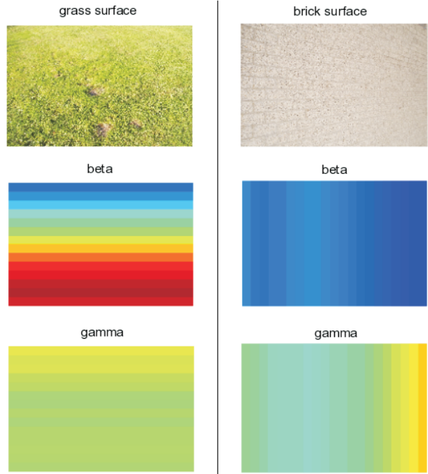
Figure 3. Natural image statistics-based Weibull distribution: parameter values as a function of depth for textures of grass (left column) and wall bricks (right column): \beta decreases from the point of fixation, whereas \gamma increases with depth. The color map has been hard-limited to a pre-defined range, such that results are comparable to each other.
