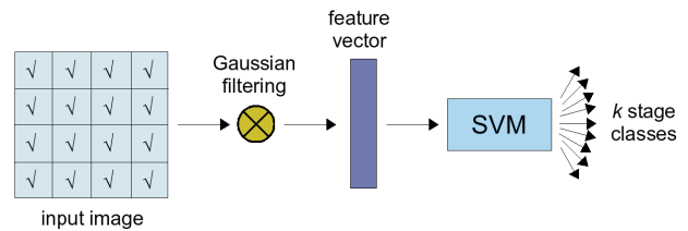
Figure 5. A simplified block-diagram of classification with Support Vector Machines: a generic stage detector is defined on the 4 \times 4 region grid - features extracted from image regions are input into the SVM directly.
