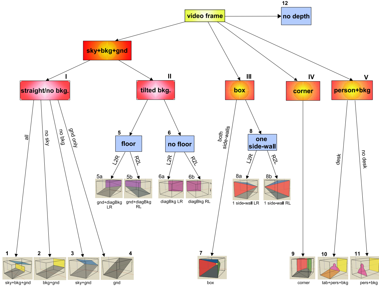
Figure 4. Hierarchical classification into stages: the classes of the intermediate hierarchy level are represented by Roman numerals I-V, whereas those of the lowest level are represented in Arabic numerals 1 through 12. Note that the symmetry of certain stages is represented by additional division into sub-stages.
