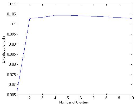
Fig.7: The data likelihood as a function of the number of clusters.
