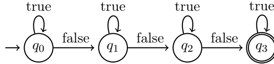
Figure 2: This finite automaton recognizes whether at least 3 sentences in the text are false. This automata needs 4 states. It starts in the rejecting state, q_0 , and eventually, if the condition is satisfied, moves to the accepting state, q_3 . Furthermore, notice that to recognize “at least 8” we would need 9 states and so on.
