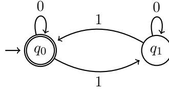
Figure 3: Finite automaton checking whether the number of “1”s is even.
