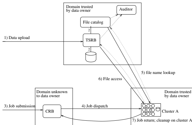
Figure 2. Proposed framework: files, file names and metadata are managed by a Trusted SRB. Dotted lines depict microcontract establishment and auditing, solid lines depict data flow and job transfers. See text.
