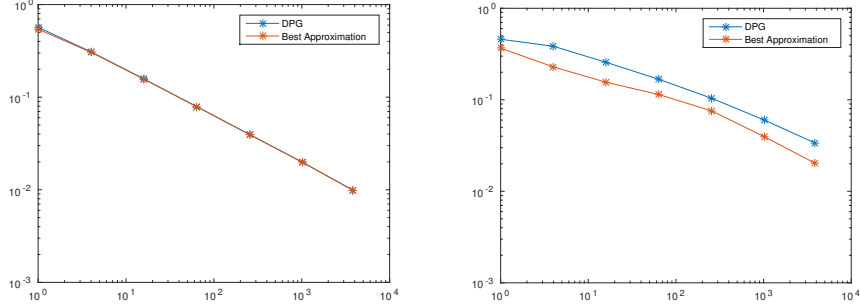
FIGURE 2. L_2(\Omega) -error in u_H and that in the best approximation versus 1/h^2 ( \approx \dim \mathcal{U}_H ), for f(\mathbf{x}) = 1 - x_1 , \mathbf{b} = (1, 1)^\top (left) and \mathbf{b} = (1, \frac{1}{16})^\top (right).
