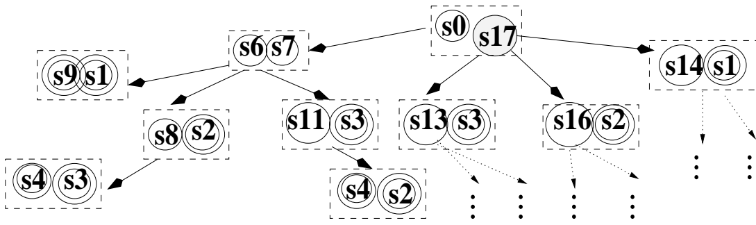
Figure 5: A portion of the backoff graph for the subtrees in Figure 3
