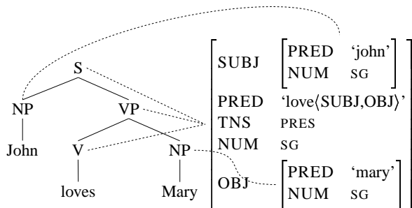
Figure 6: An LFG representation for John loves Mary .
