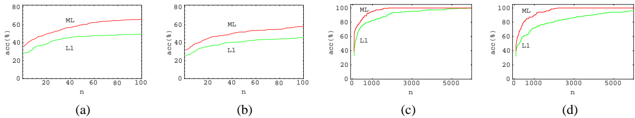
Figure 7: Retrieval accuracy using L_1 (L1) and the maximum likelihood distortion measure (ML): HSV (a)-(c), RGB (b)-(d)
