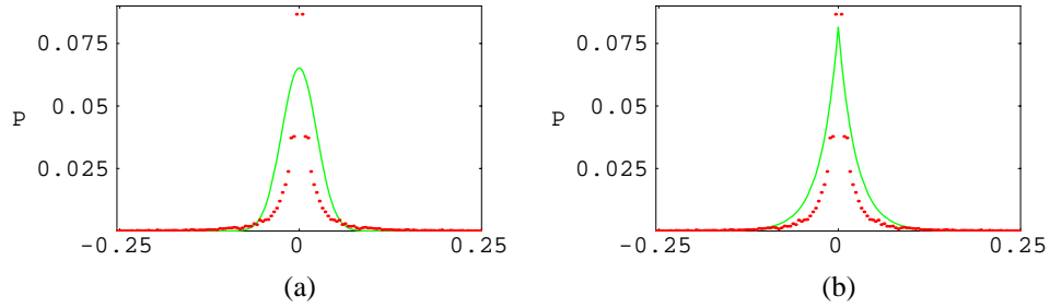
Figure 3: Similarity noise distribution in HSV compared to best fit Gaussian (a) (modeling error is 0.106) and best fit exponential (b) (modeling error is 0.082)
