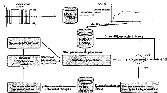
Fig. 2 Function blocks of the FEM->HDL-A translator
