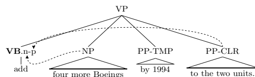
(a) An NP PP subcategorization frame on the verb ‘add’.
