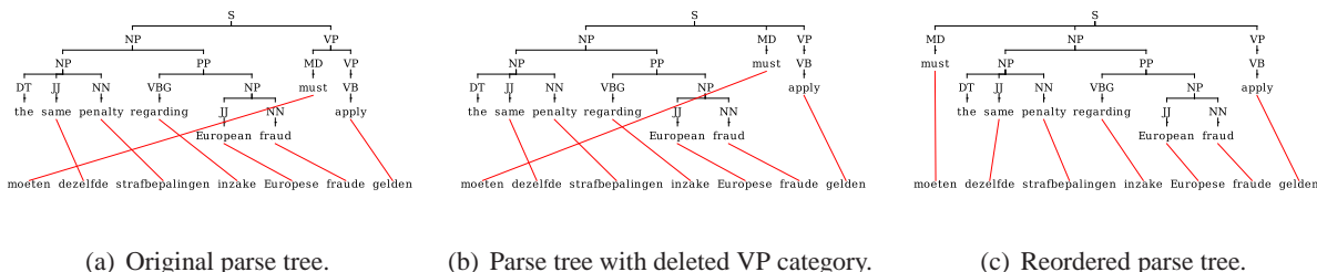
Figure 3: Example of text monotonicization with tree transformation.
