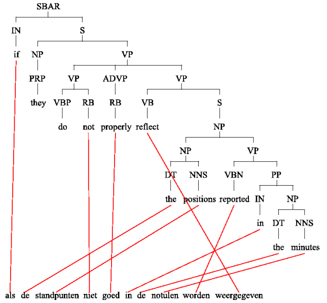
Figure 4: Example of unfoldable alignment crossings.
