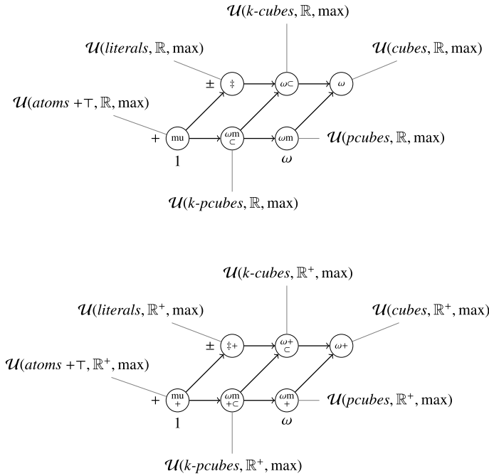
Fig. 1. Summary of expressivity results.
