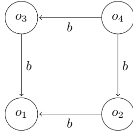
Figure 3. A plausibility model \mathcal{M}_2 for G which is not a “game model” (see below)
