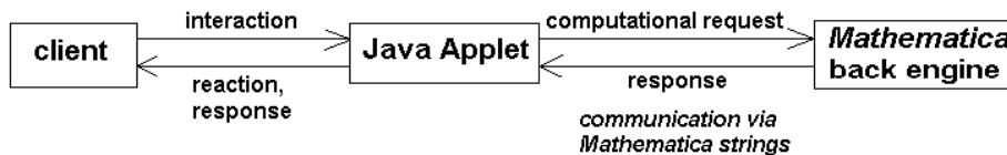
Figure 8. The general scheme of the Mathematica empowered architecture
