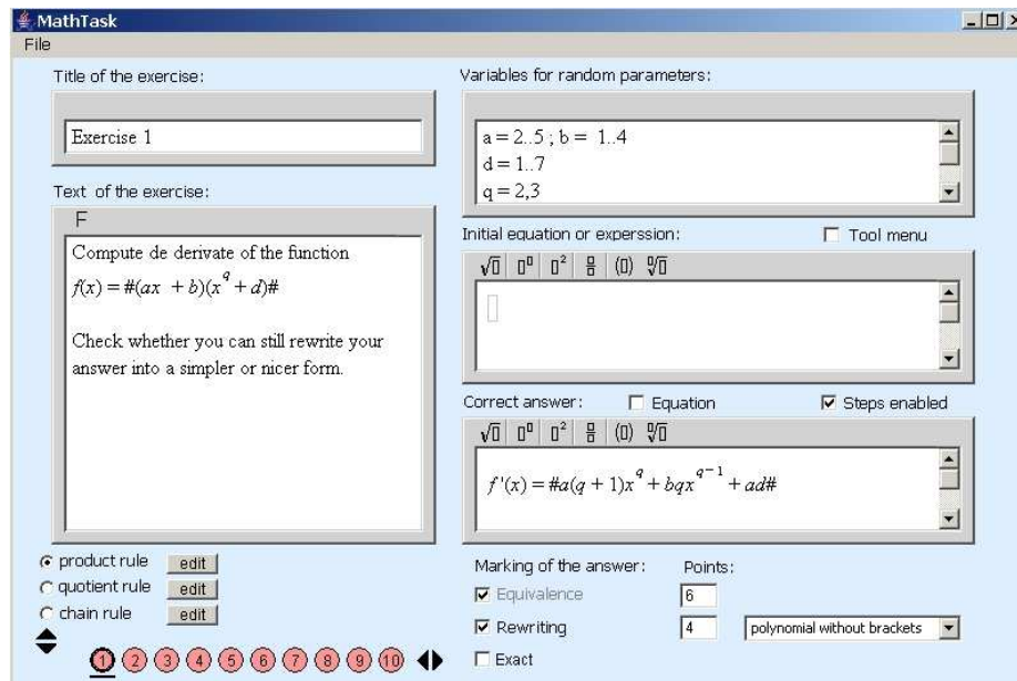
Figure 7. Creation of an exercise with (the prototype of) the applet generator.
