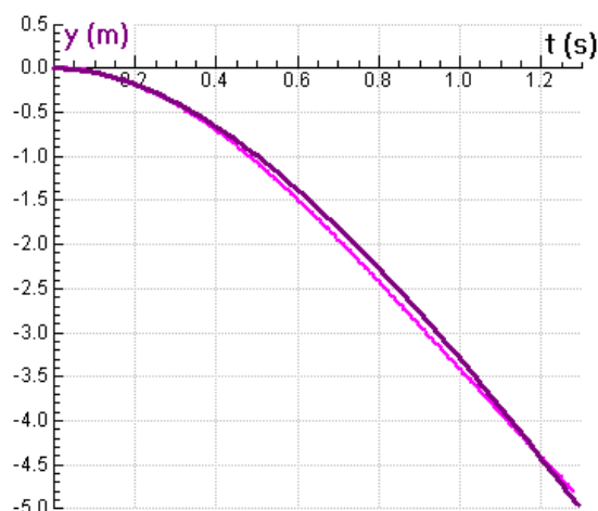
Fig 5. The position-time graph of the best simulation for the linear drag model.
