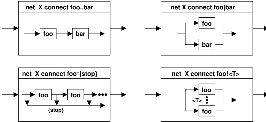
Fig. 2. Illustration of network combinators and their operational behaviour: serial composition (top-left), parallel composition (top-right), serial replication (bottom-left) and indexed parallel replication (bottom-right)
