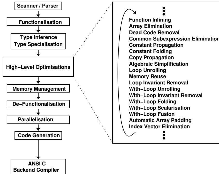
Figure 4. Organisation of the SAC compiler tool chain
