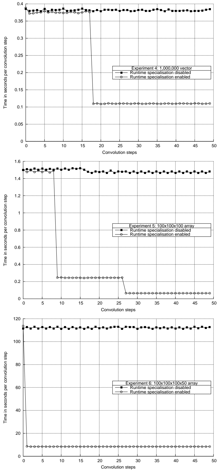
Figure 10. Experimental results obtained by applying the case study code discussed in Section 3 to a vector, a tensor and a 4-dimensional array with runtime specialisation disabled and enabled
