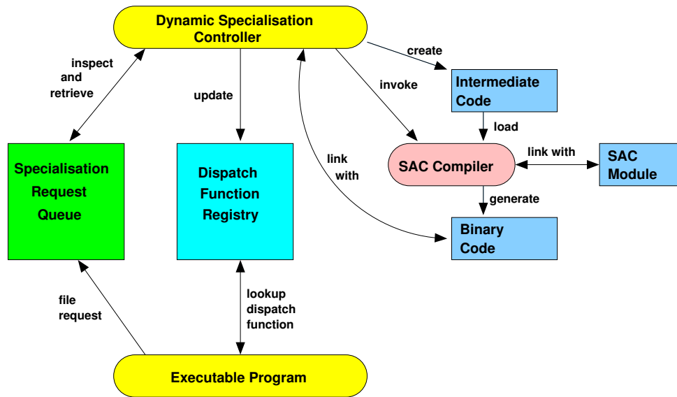
Figure 6. Architecture of our adaptive compilation framework
