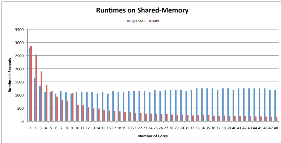
Fig. 26. Runtimes on a 48-core shared-memory machine using MPI and OpenMPI
