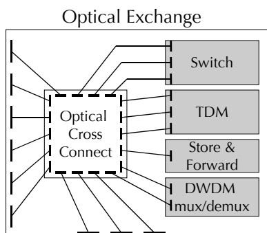
Figure 3. Possible implementation of an Optical Exchange with an Optical Cross Connect at the core and providing miscellaneous services.
