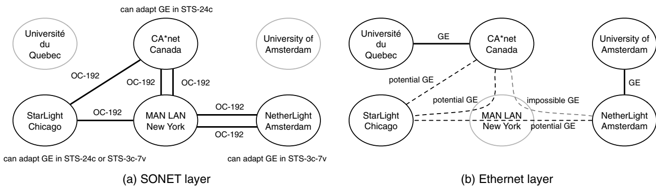
Fig. 2. Two layers (SONET and ethernet, respectively) of the multi-layer network of Fig. 1. This still does not visualise the adaptations between the two layers.
