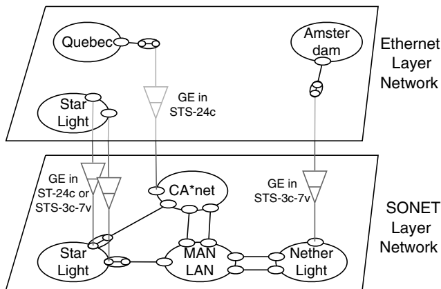
Fig. 4. The network of Fig. 1, modelled as functional elements.
