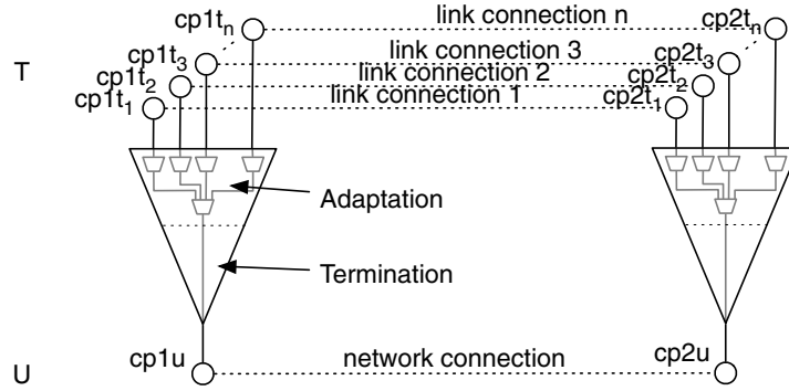
Fig. 6. Channels correspond with multiple link connections at the client layer over one link connection at the server layer.
