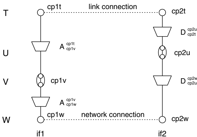
Fig. 9. Example of a well typed, but invalid connection. U and V are different layers.
