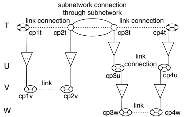
Fig. 8. Example of a valid network connection. A valid tandem connection consisting of two link connections and a matrix connection.
