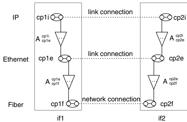
Fig. 5. Example of a multi-layer network connection. Interfaces if1 and if2 are modelled as connection points at all three layers. The relation between the connection points is defined by the adaptation and termination functions.
