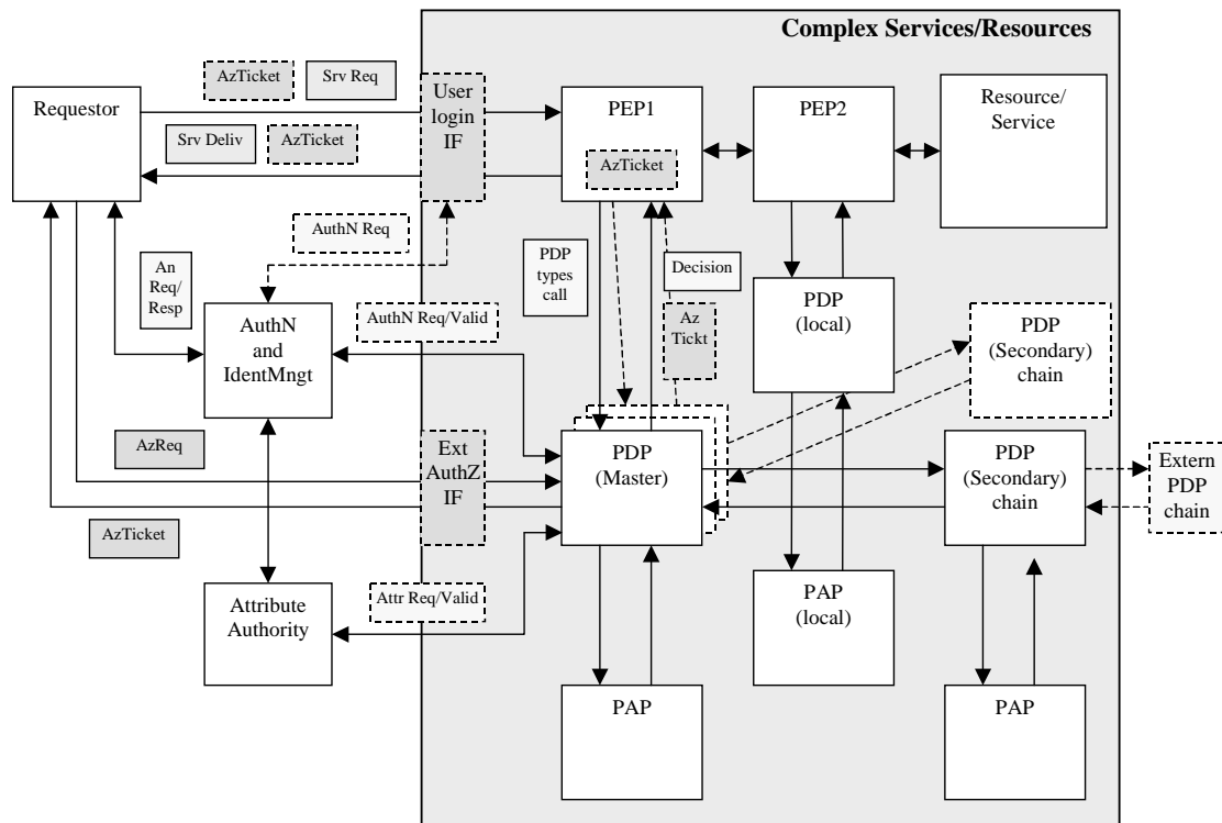
Figure 4. Multiple/multi-domain policies combination in complex resource/service Authorisation service (combined pull-push model)
