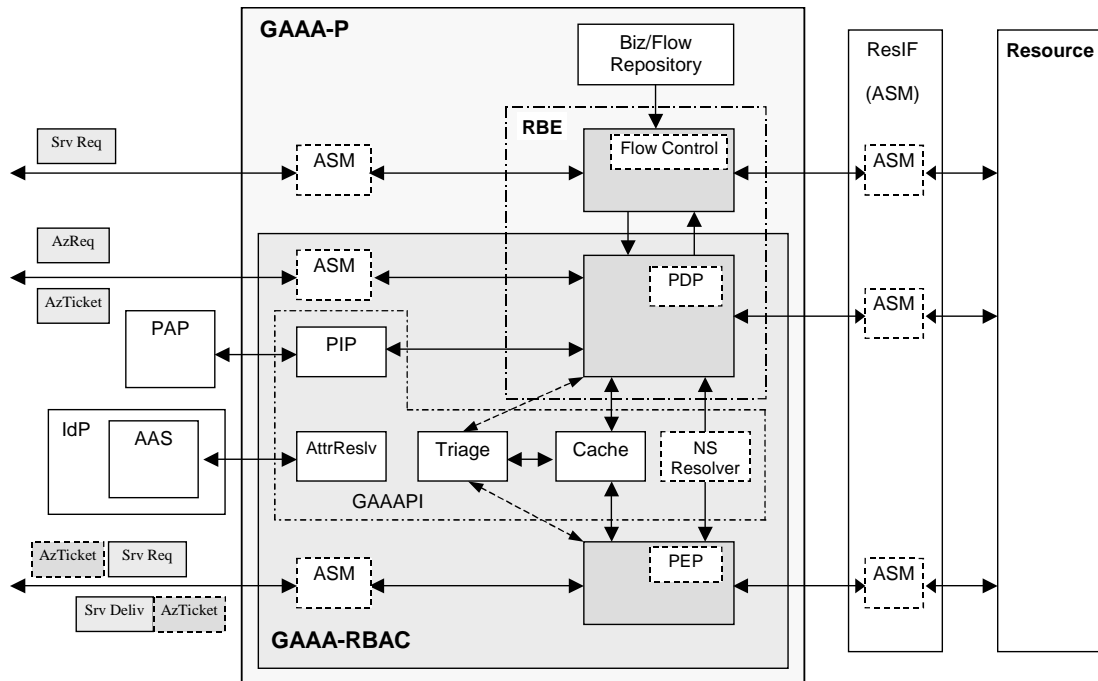
Figure 6. GAAA-P and GAAA-RBAC structure and main functional components
