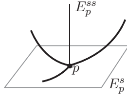
Figure 9: Sketch of the heteroclinic trajectories approaching p in Case 9, with G = \mathbb{D}_3 .
