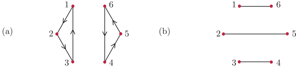
Figure 6: Markov graphs representing the non-wandering shift dynamics on either side ((a) and (b)) of the bifurcation point in Case 11 of Table 2, with G = \mathbb{D}_3 .
