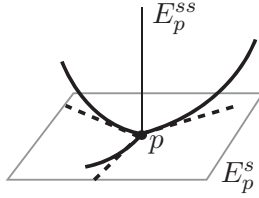
Figure 7: Sketch of the homoclinic connections approaching p in Case 6, with G = \mathbb{D}_3 .
