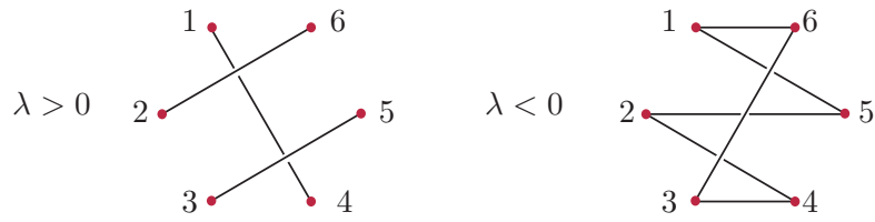
Figure 11: Symbolic dynamics in region I of Figure 10.
