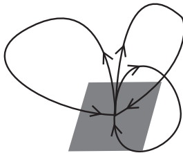
Figure 1: Illustration of three homoclinic trajectories approaching p when \dim(E_p^s) = 2 . Note that the state space has to be at least four dimensional.
