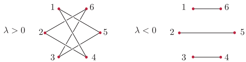
Figure 12: Symbolic dynamics in region II of Figure 10.
