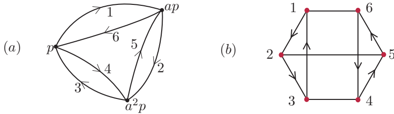
Figure 4: (a) Schematic representation of the connections of a relative homoclinic cycle with G = \mathbb{D}_3 , G_p = \mathbb{Z}_2 and G_\gamma = \{id\} . (b) Markov graph representing the non-wandering shift dynamics that exists on one side of the homoclinic bifurcation, in the case of trivial representation of G_p on E_p^s (Case 10 of Table 2) .
