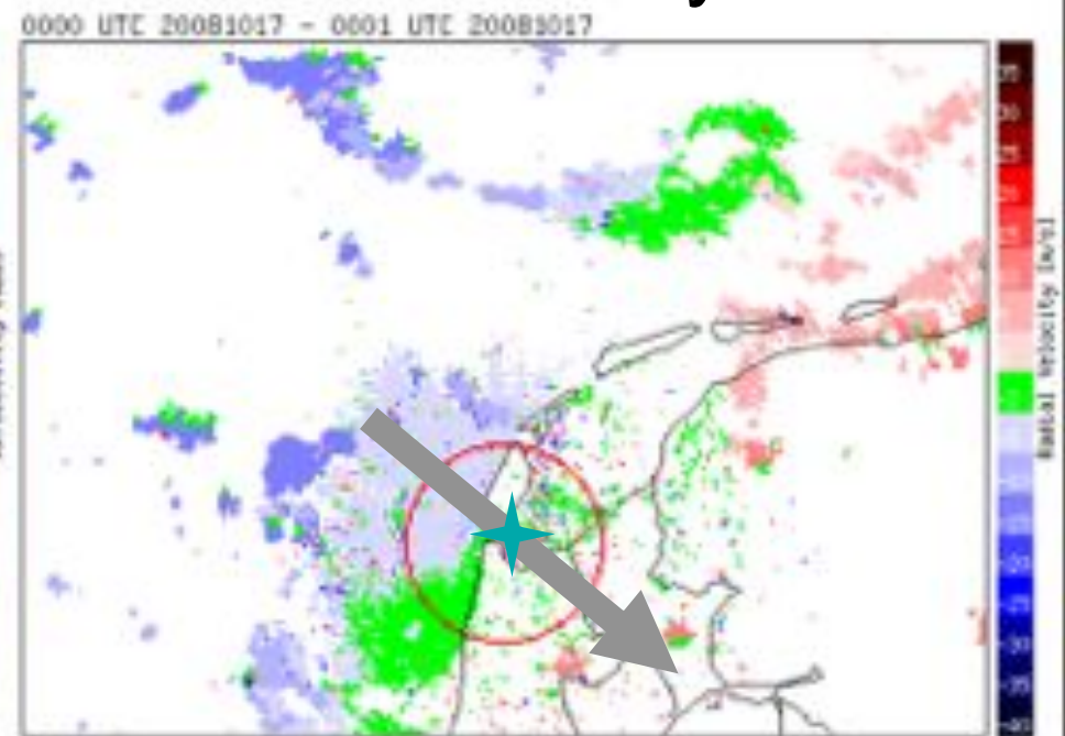
radial velocity
