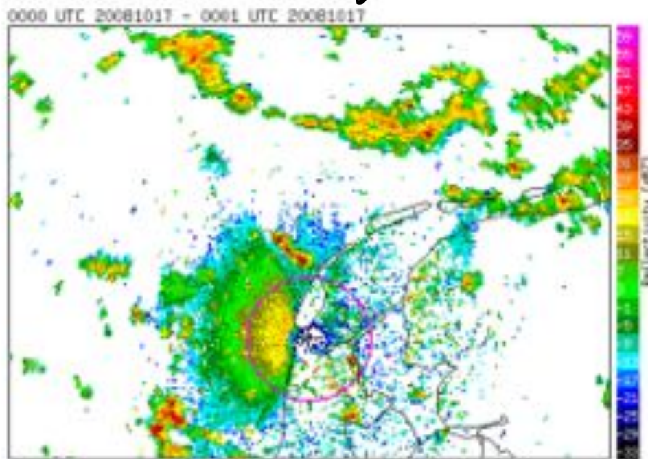
reflectivity factor
